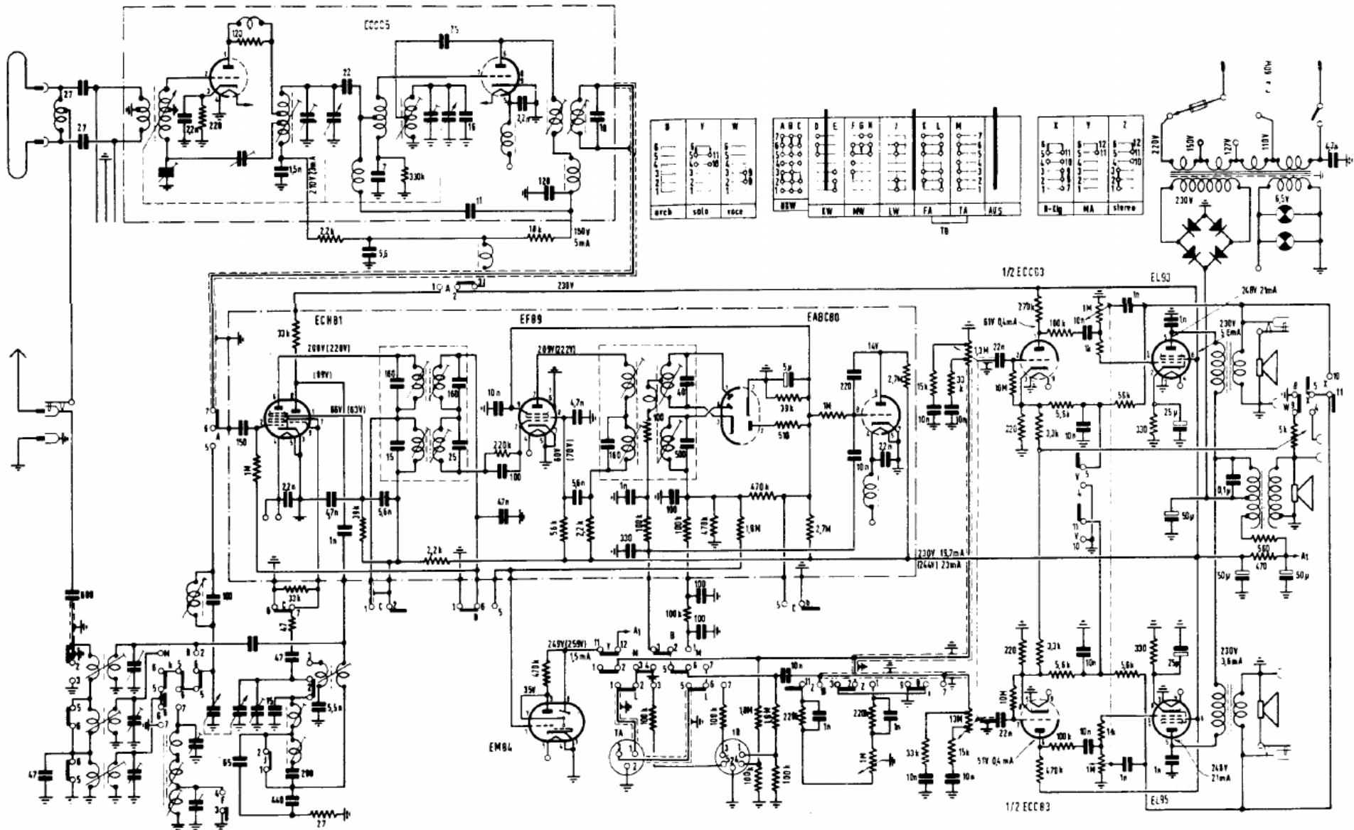
PHILCO mod. BELFAST
